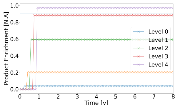
Fig. 3. Evolution of the different product assays at each cascade level for the case 2 without recycling.
